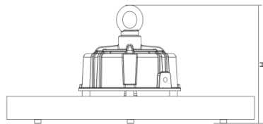
SHB25/80 SHB25/120 - 320mm dia x 120mm hm
